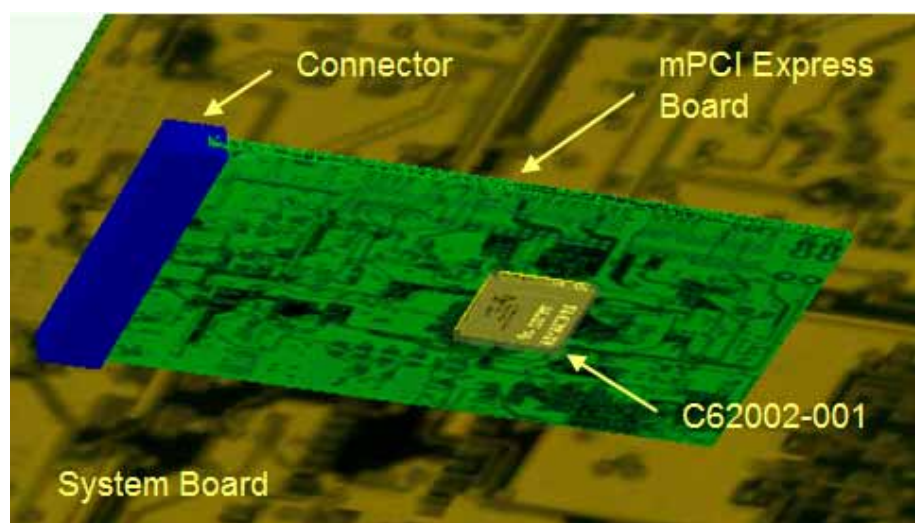
Figure 84. 82574 Test Setup
