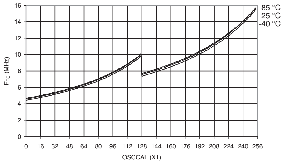
Figure 27-25. Calibrated 8 MHz RC Oscillator Frequency vs. OSCAL Value
